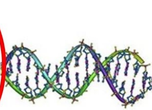
NUCLEIC ACIDS
