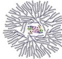
CARBOHYDRATES
